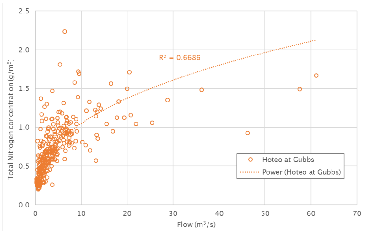
Figure 39 - Comparison of Total Nitrogen concentration (mg/L) and daily flow (m 3 /s) at Hōteo at Gubbs
